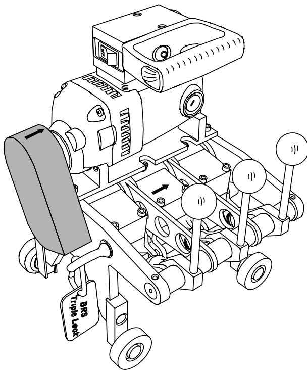
CCG Motor Seaming Machine
